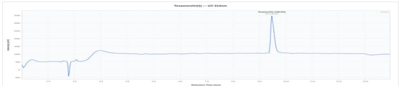
Tesamorelin 10mg - NRTESA10-0021: UV Chromatogram
